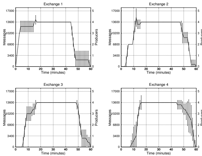
Fig. 7. Number of messages processed by the 4 queue exchanges. The plots depict the mean values and standard deviation computed on 5 independant runs. At the beginning, only Exchange 1 is active. As producers connect to the queue and the load increases, Exchanges 2,3 and 4 are started by the rules and scaling management. The second y-axis on the right depicts the number of users connected to an exchange corresponding to a processed number of messages.
